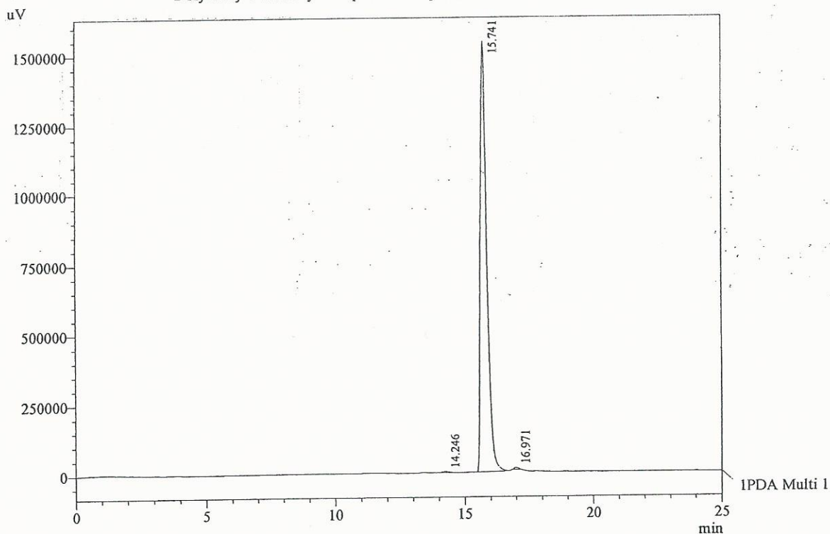
Chromatogram 2-Hydroxy-6-methoxy acetophenone D:\promonence
