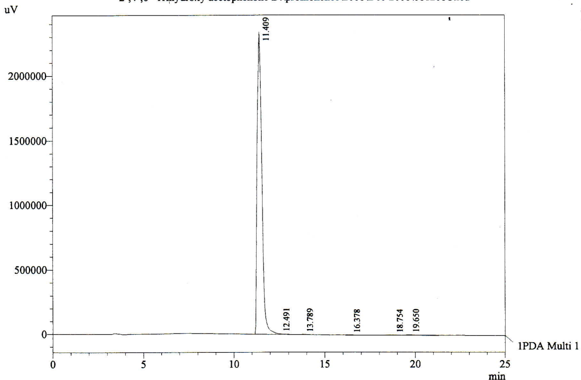
Chromatogram 2',4',6'-Trihydroxy acetophenone D:\promonence\2008\Dec-2008\081208C.lcd
